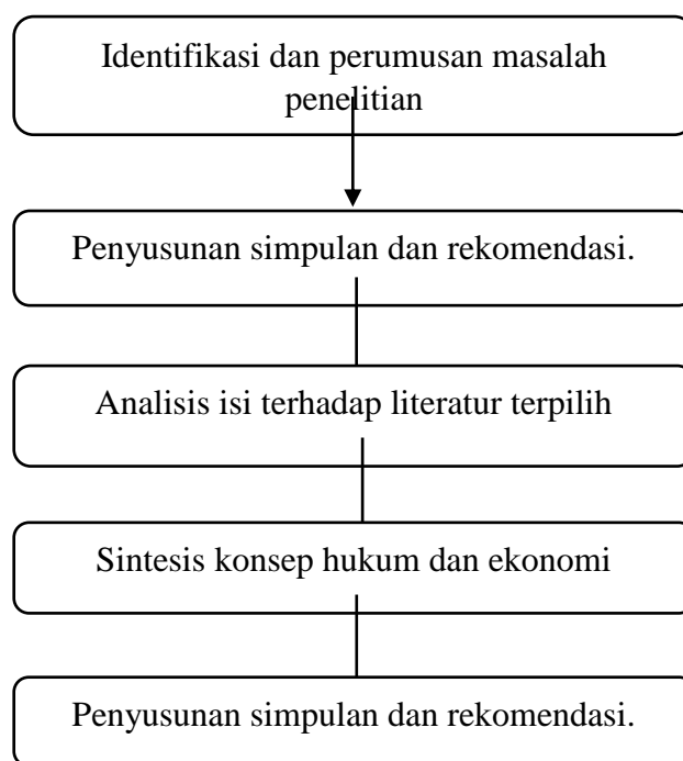
Gambar 1. Alur Penelitian
