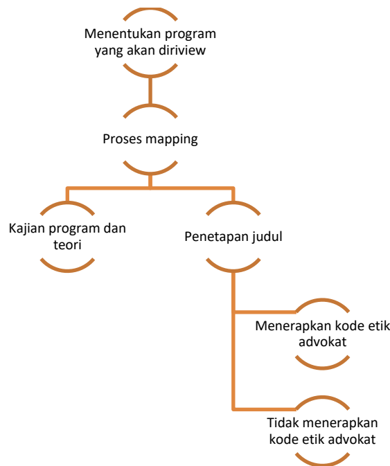
Gambar 1. Alur Penelitian
