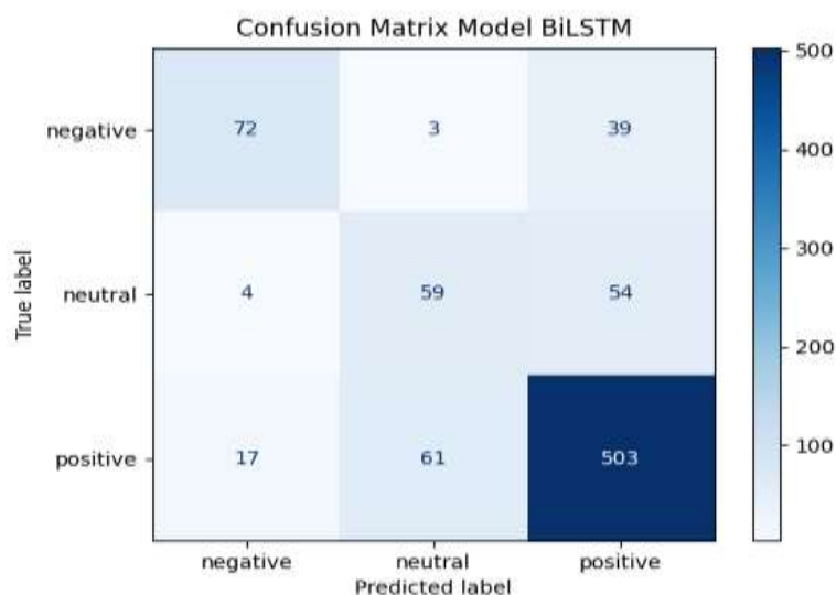
Gambar 5. Confusion Matrix Model BiLSTM
