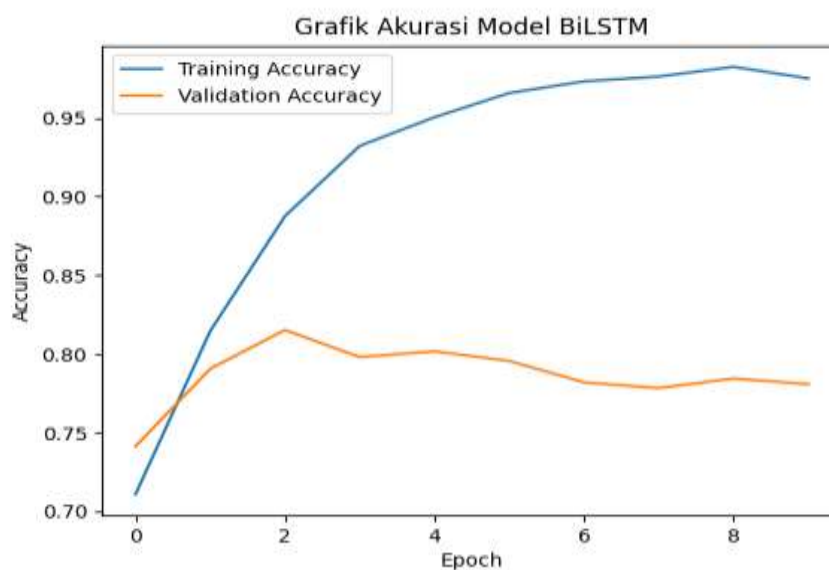
Gambar 3. Grafik Accuracy Training dan Validation per Epoch
