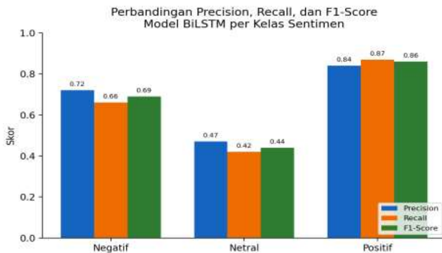
Gambar 6. Perbandingan Precision, Recall, dan F1-Score per Kelas Sentimen
