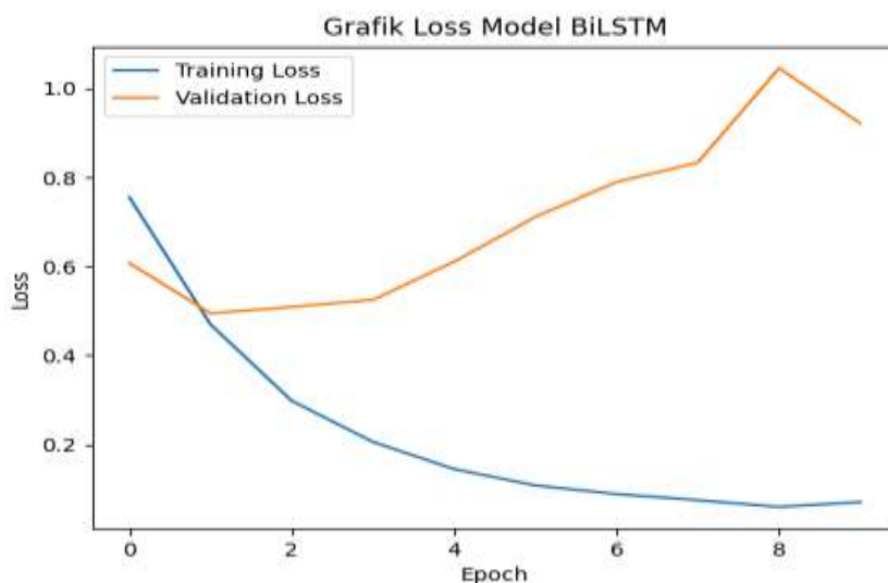
Gambar 4. Grafik Loss Training dan Validation per Epoch
